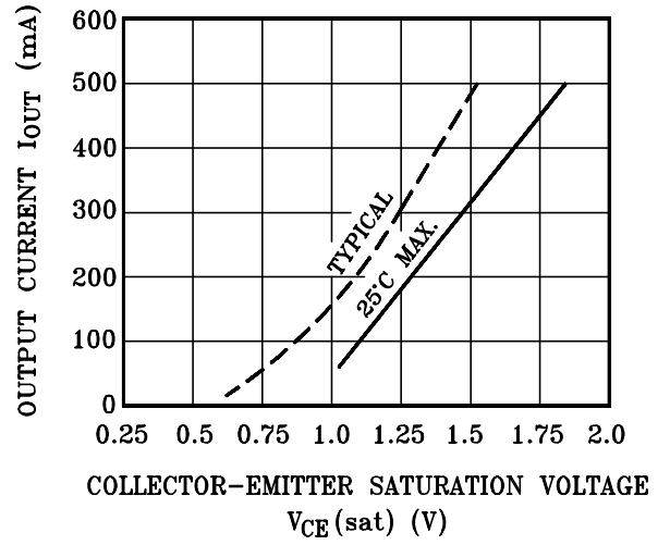
I_{OUT} - V_{CE(sat)}
