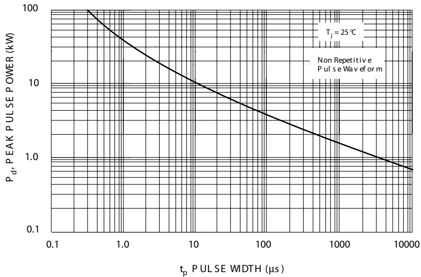
Fig 3 Pulse Rating Curve
