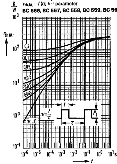
Permissible pulse load r_{thJA} = f(t); v = \text{parameter}
