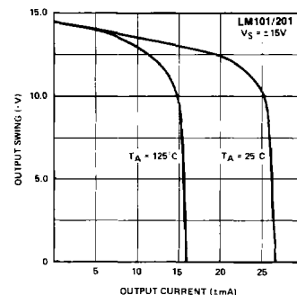
CURRENT LIMITING
