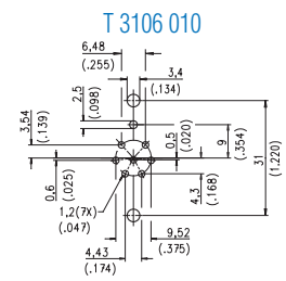
Hole pattern on PCB
