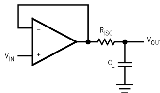
Figure 36. Compensation by Isolation Resistor
