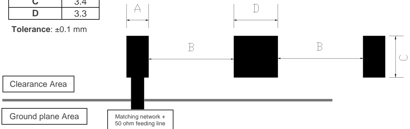
Figure 10 – Footprint dimensions for the double booster.
