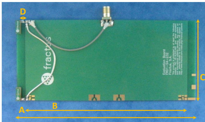
Figure 5 – EB_FR01-S4-232-UFL2R-1P. Evaluation Board 1 port providing operation in 2 frequency ranges, 824 – 960MHz and 1710 – 2690MHz.
