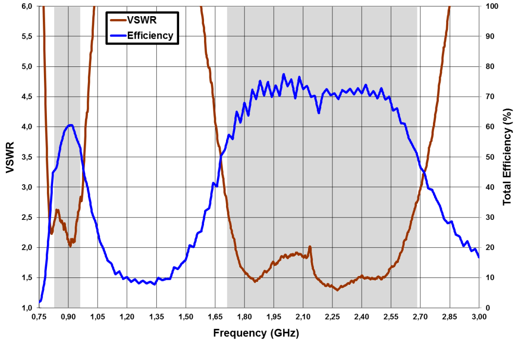
Figure 7 – VSWR and Total Efficiency for the 824 – 960 MHz frequency range and for the 1710 – 2690 MHz frequency range (from the Evaluation Board) (Figure 5).
