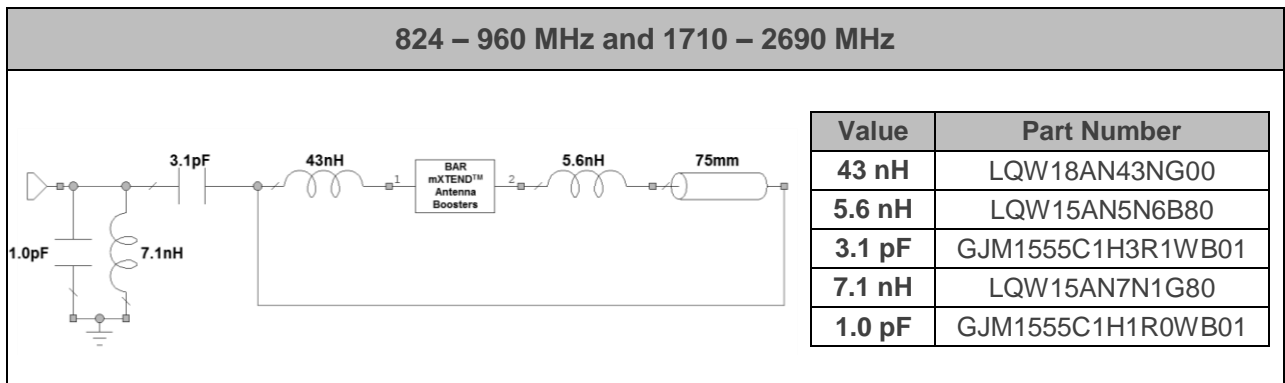
Figure 6 – Matching network implemented in the Evaluation Board 1 port (Figure 5).
