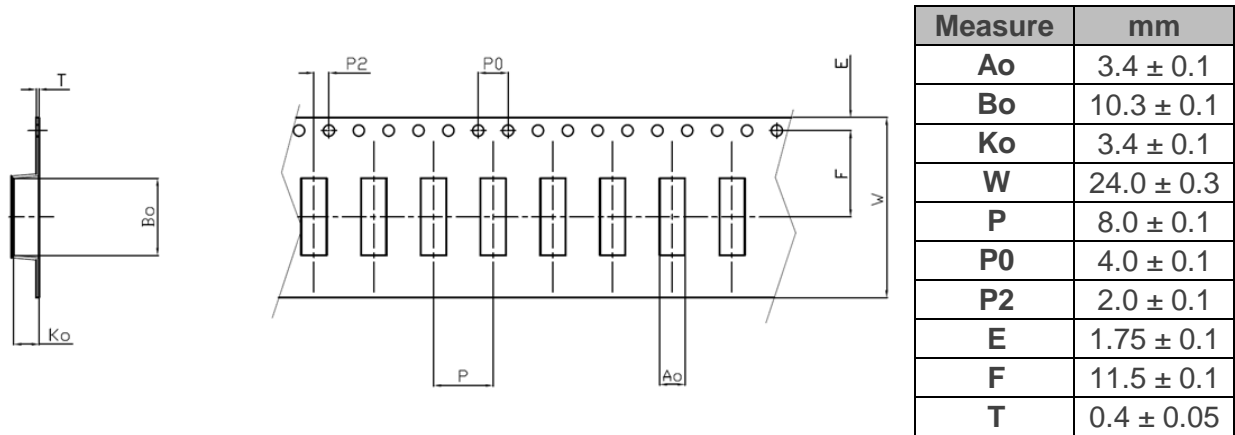
Figure 14 – Tape dimensions and Tolerances.
