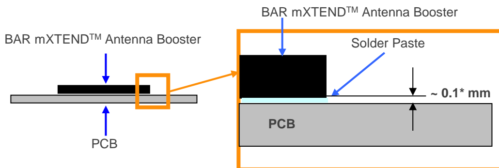
Figure 12 – Soldering Details.
