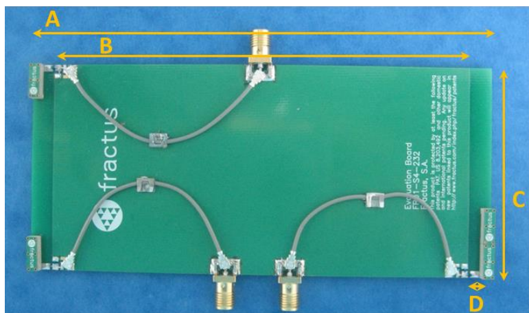
Figure 1 – EB_FR01-S4-232-UFL3R. Evaluation Board providing operation in 3 frequency ranges, 698 MHz to 798 MHz, 824 MHz to 960 MHz, and 1710 MHz to 2690 MHz.
