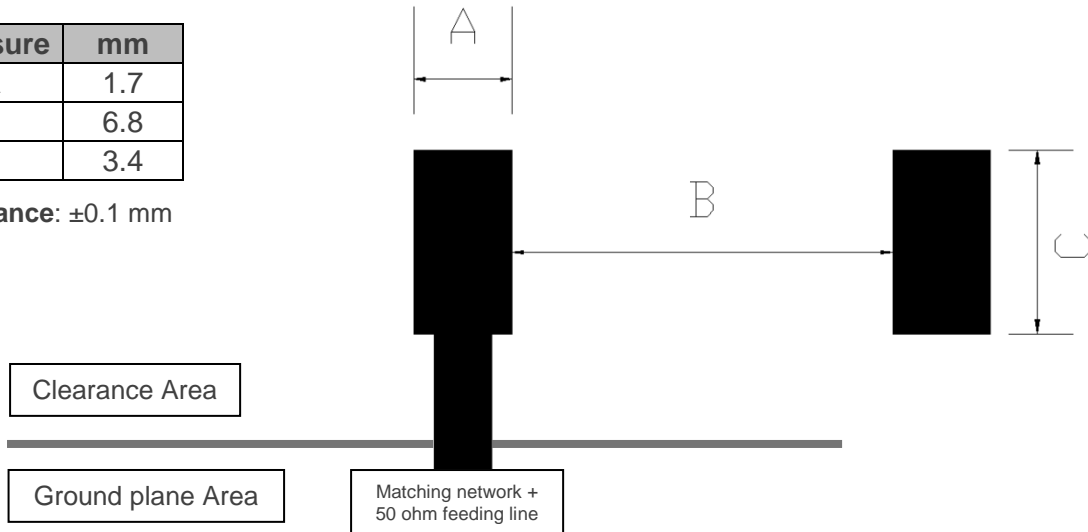
Figure 9 – Footprint dimensions for the single booster.
