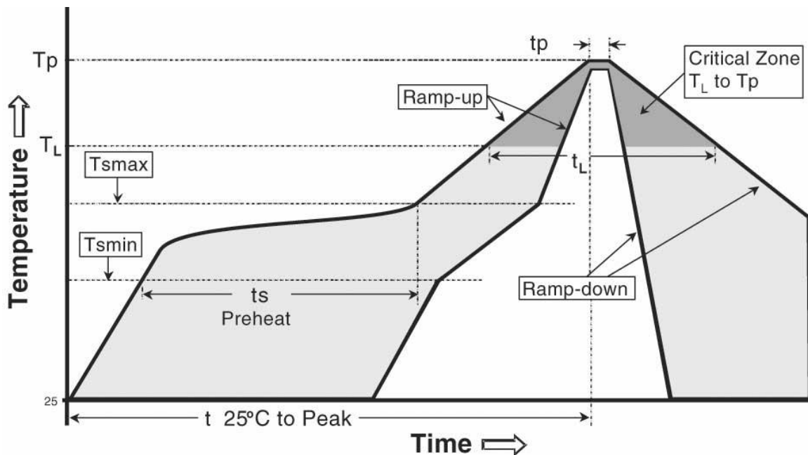
Figure 13 – Temperature profile.
