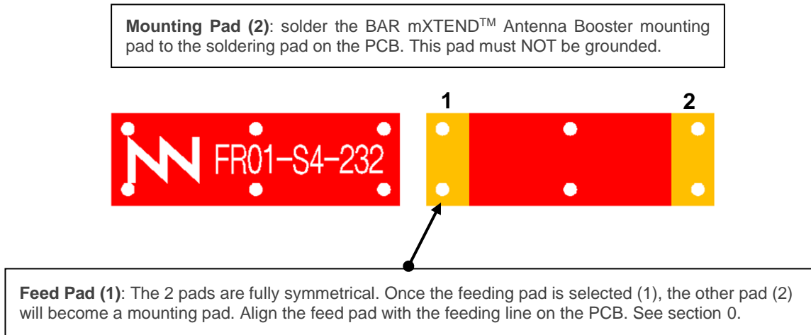
Figure 11 – Pads of the BAR mXTEND™ Antenna Booster FR01-S4-232.
