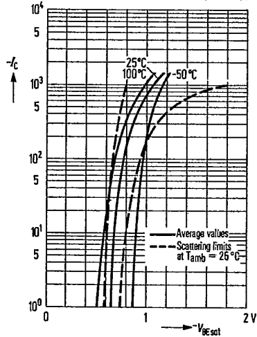
Base-emitter saturation voltage V_{BEsat} = f(I_C) h_{FE} = 10 ; T_{amb} = \text{parameter} (common emitter configuration) BD 136, BD 138, BD 140
