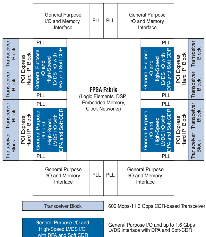
Figure 1-3. Stratix IV GT Chip View (Note 1)
