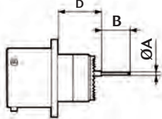
Type 2 Short square flange receptacle
