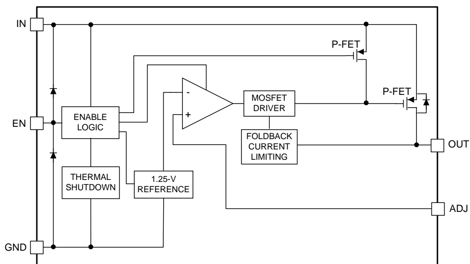
Figure 28. LP38692-ADJ (SOT-223, WSO)
