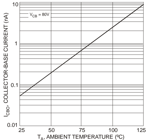
Fig. 6 Typical Collector-Cutoff Current vs. Ambient Temperature
