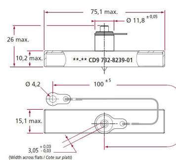
732-8239-01
