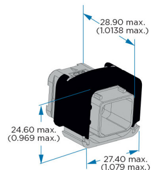
PLUG
