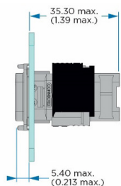
BOX MOUNTING RECEPTACLE
