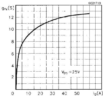
Transconductance
