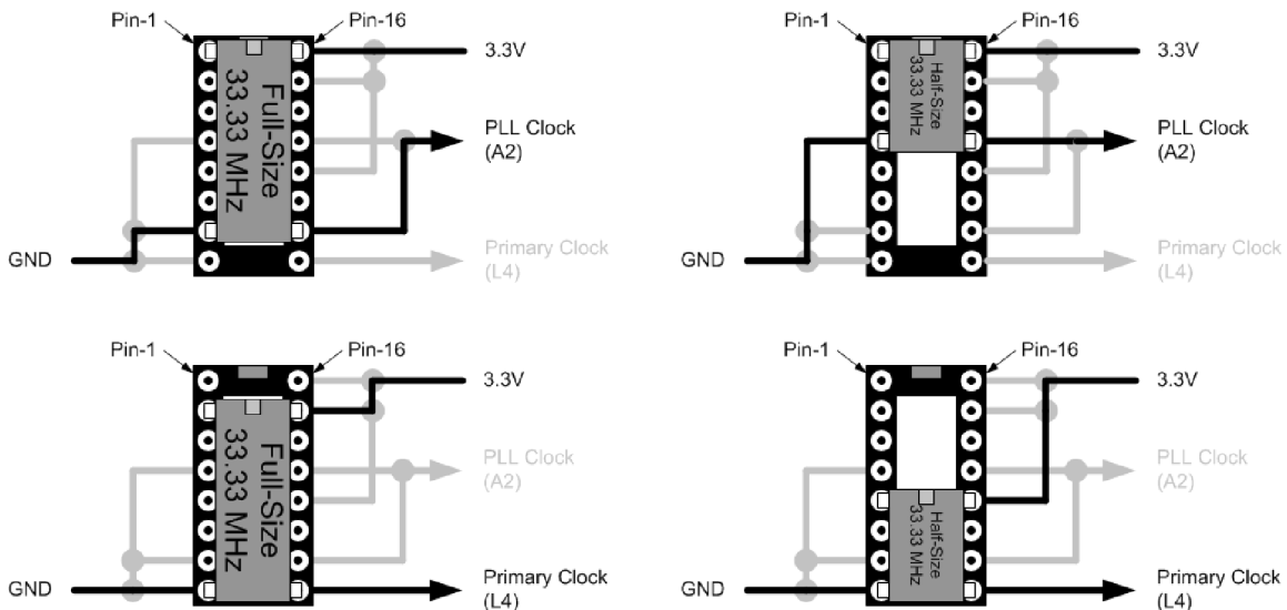
Figure 2. On-board Oscillator
