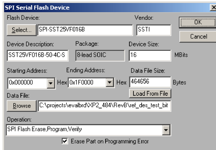
Figure 16. SPI Serial Flash Device Dialog
