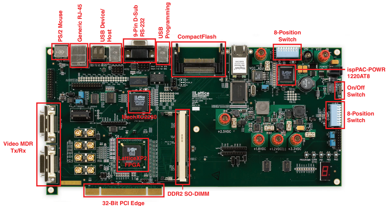
Figure 1. LatticeXP2 Advanced Evaluation Board
