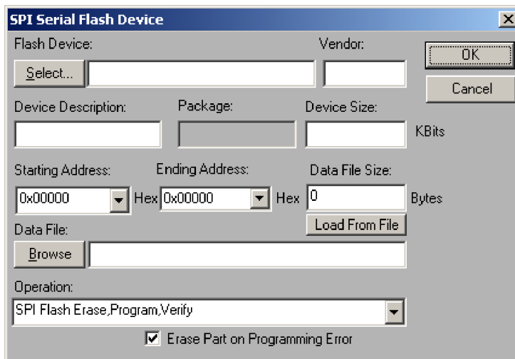
Figure 14. SPI Serial Flash Device Dialog
