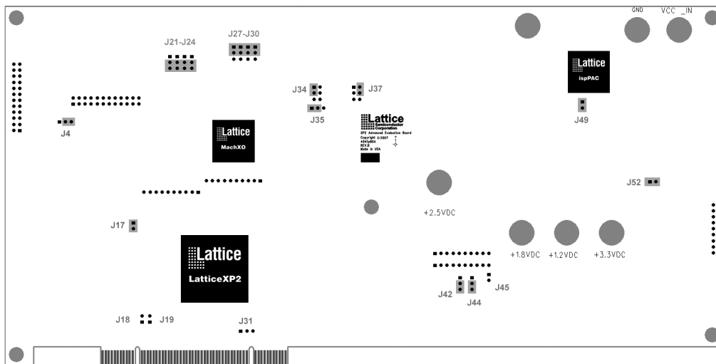
Figure 4. Default Jumper Settings
