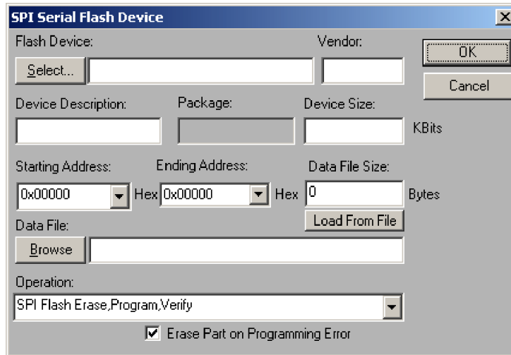
Figure 7. SPI Serial Flash Device Dialog
