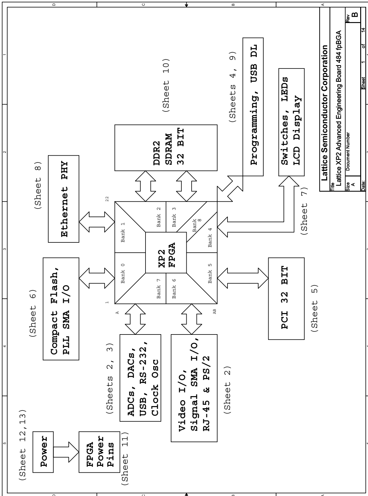
Figure 19. LatticeXP2 Advanced Evaluation Board
