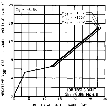
Fig. 6ee - Typical Gate Charge Vs. Gate-to-Source Voltage IRF9230
