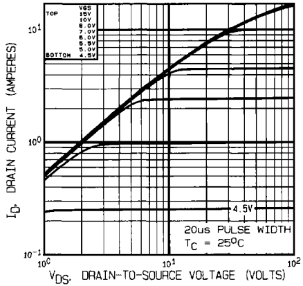
Fig. 1t - Typical Output Characteristics, T_C = 25^\circ\text{C} IRFAE30
