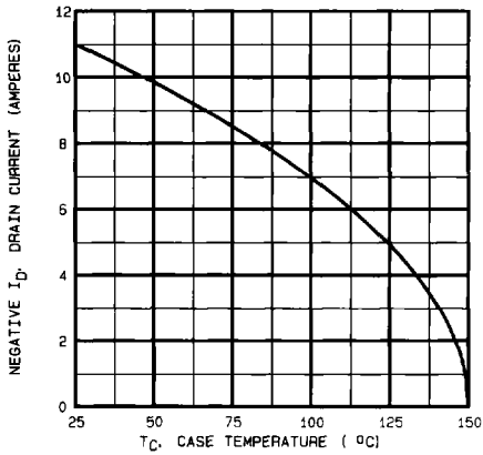
Fig. 9cc – Maximum Drain Current Vs. Case Temperature IRF9130
