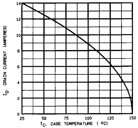
Fig. 9d - Maximum Drain Current Vs. Case Temperature IRF130
