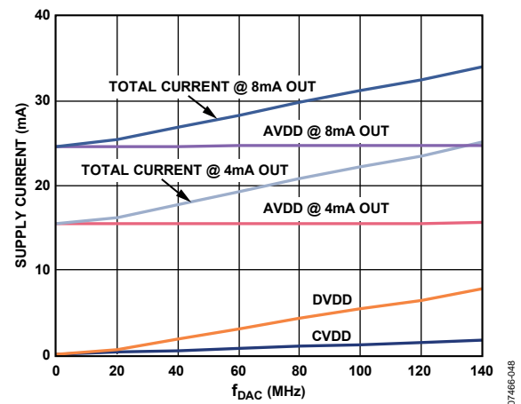
Figure 80. AD9114/AD9115/AD9116/AD9117 Supply Current vs. f_{DAC} , 1.8 V
