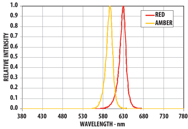
Figure 1. Relative Intensity vs. Wavelength for AllnGaP
