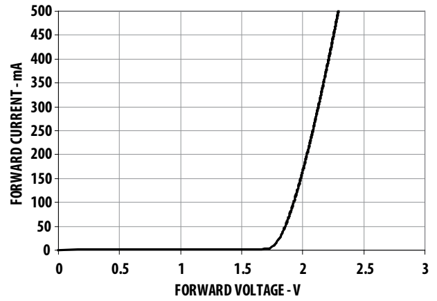
Figure 2. Forward Current vs Forward Voltage for AllnGaP
