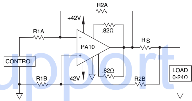
FIGURE 1. VOLTAGE-TO-CURRENT CONVERSION
