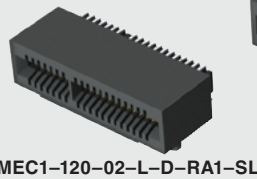
MEC1-120-02-L-D-RA1-SL
