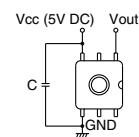
Terminal connection diagram
