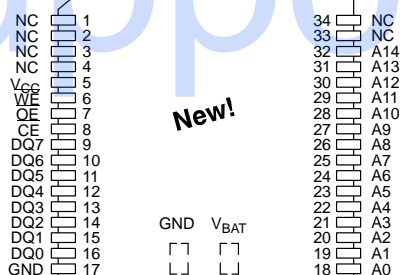
34-PIN POWERCAP MODULE (PCM) (USES DS9034PC POWERCAP)
