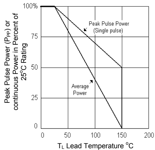
FIGURE 3 Derating Curve
