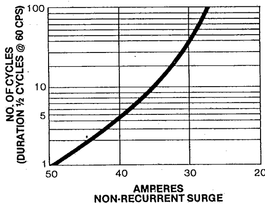
FIG. 4 MAXIMUM SURGE CURRENT
