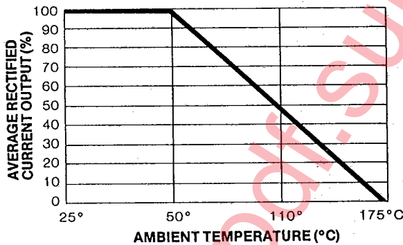
FIG. 1 MAXIMUM CURRENT OUTPUT VS. AMBIENT TEMPERATURE
