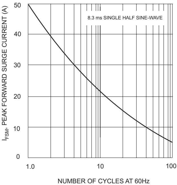
NUMBER OF CYCLES AT 60Hz Fig. 3 Maximum Non-Repetitive Peak Forward Surge Current
