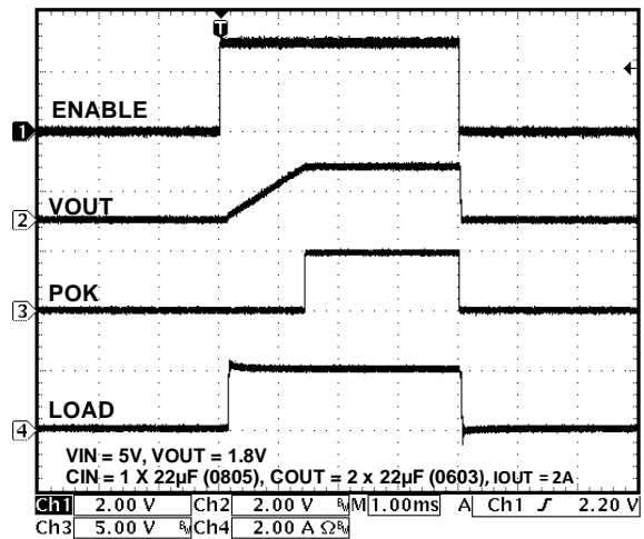
Startup Waveforms at 2A
