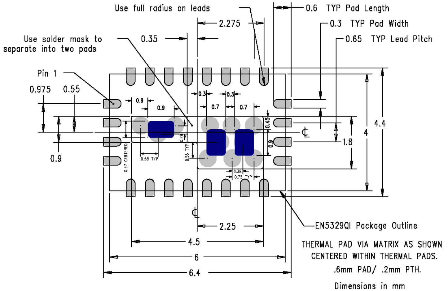
Figure 11. EN5329 PCB Footprint (Top View)
