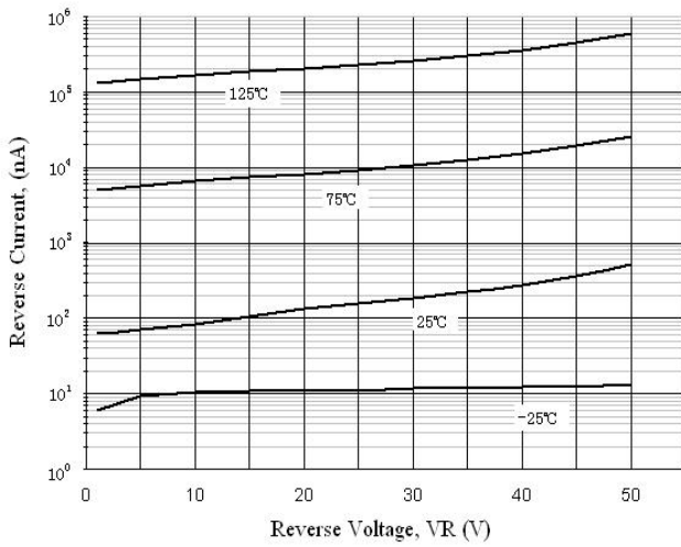
Fig.3 Reverse Current vs Reverse
