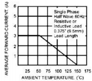
FIG.2- MAXIMUM FORWARD CURRENT DERATING CURVE
