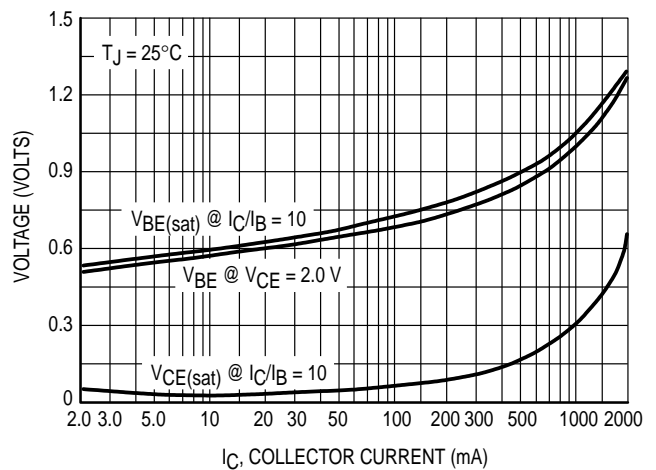
Figure 11. "On" Voltage
