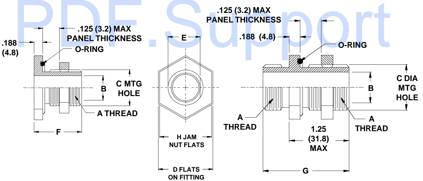
Bulkhead Adapters 710-100/101/372
