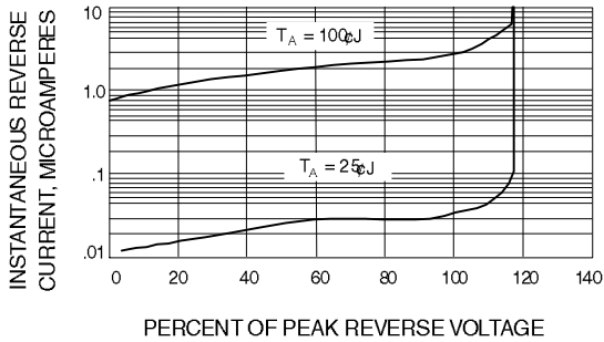
Fig. 3-TYPICAL REVERSE CHARACTERISTICS
