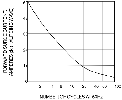
Fig. 4-NON-RECURRENT SURGE RATING
