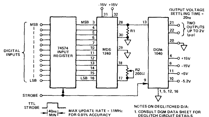
Figure 14. Ultra High-Speed Deglitched D/A
