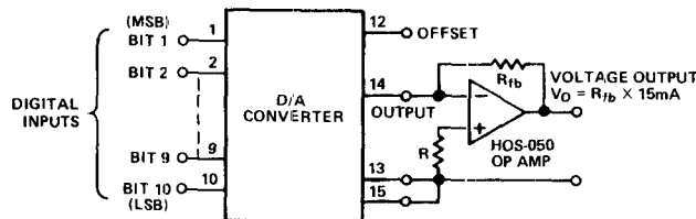
Figure 11. Voltage Output
