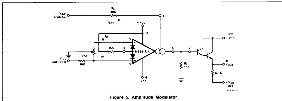
Figure 5. Amplitude Modulator
