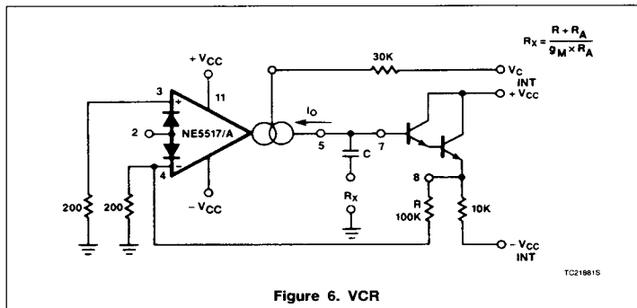
Figure 6. VCR
