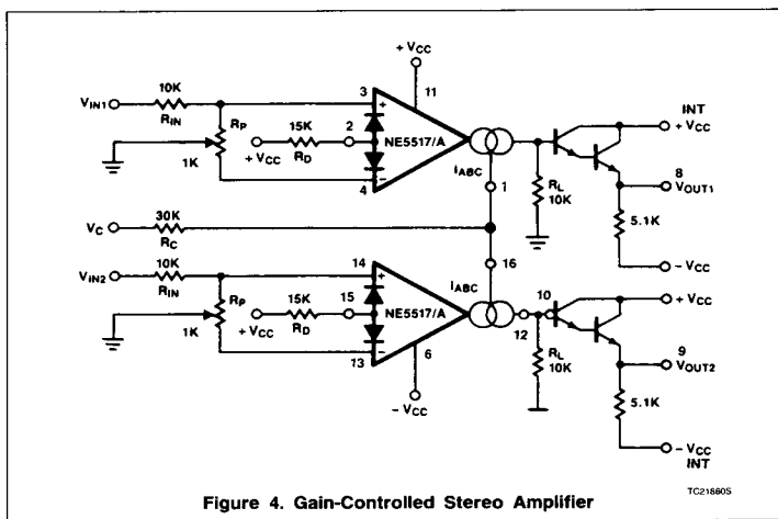
Figure 4. Gain-Controlled Stereo Amplifier
