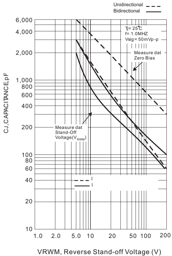
Fig.4 TYPICAL CAPACITANCE
