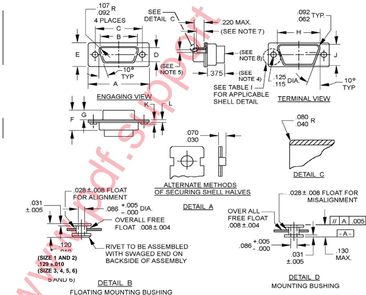
FIGURE 1. Shell, plug, crimp type.
