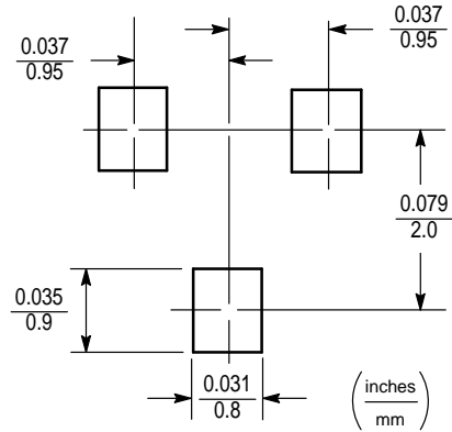
SOT-23 Footprint
